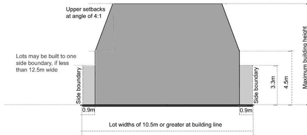
Figure D2.07: The following building envelope applies to lots with a width measured at the building line of 10.5m or greater
