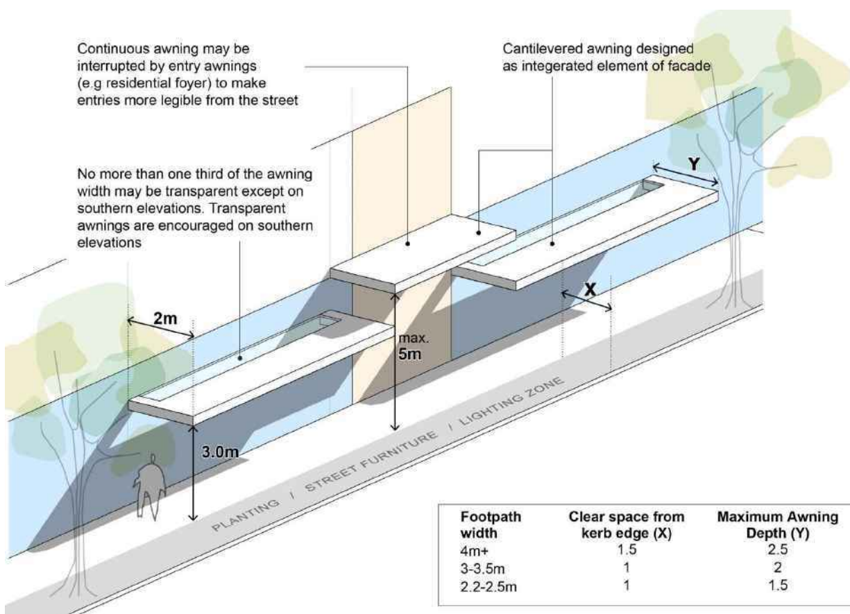
Figure F4E8.32: Awnings diagram
