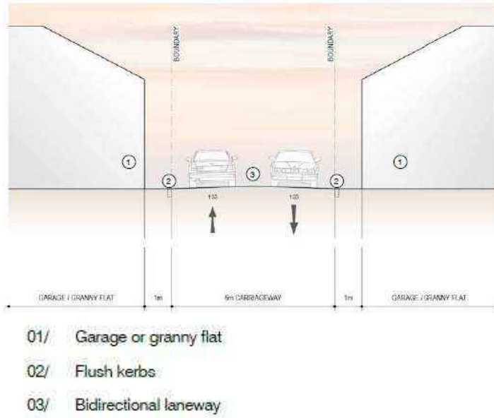
Figure F2E6.06: Road type 4 typical section
