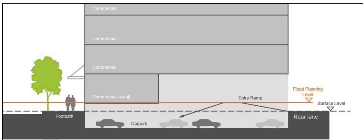
Figure B1(a).0201: Basement ramp design to minimise inundation
