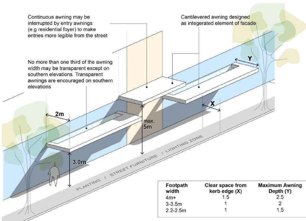
Figure F4E8.12: Awnings diagram
