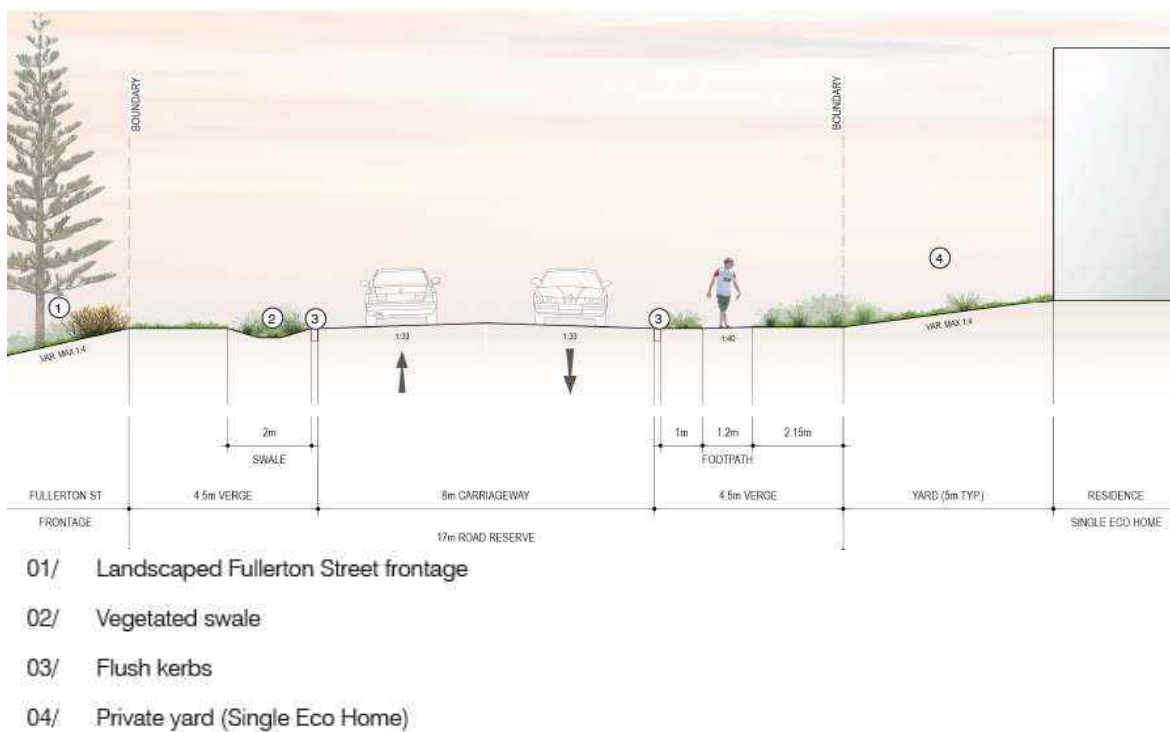
Figure F2E6.03: Road type 1 typical section
