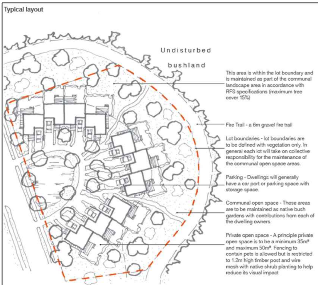
Figure F2E6.10: Area 1 Dune edge cluster housing typology
