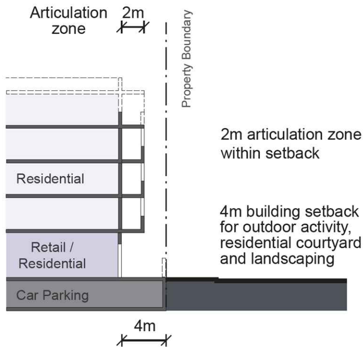
Figure E8.60: Setback transition - residential
