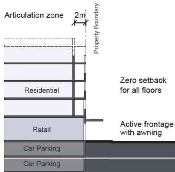
Figure F4E8.44: Setback AR1, 4-5 storeys – Corner sites/ general
