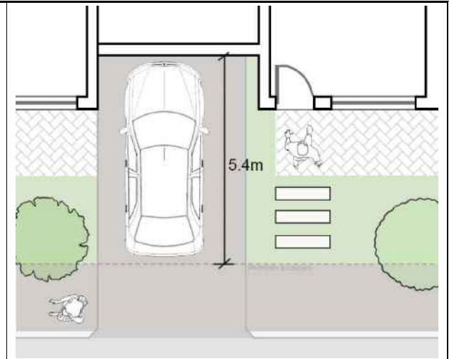
Figure C1.03: Tandem space
