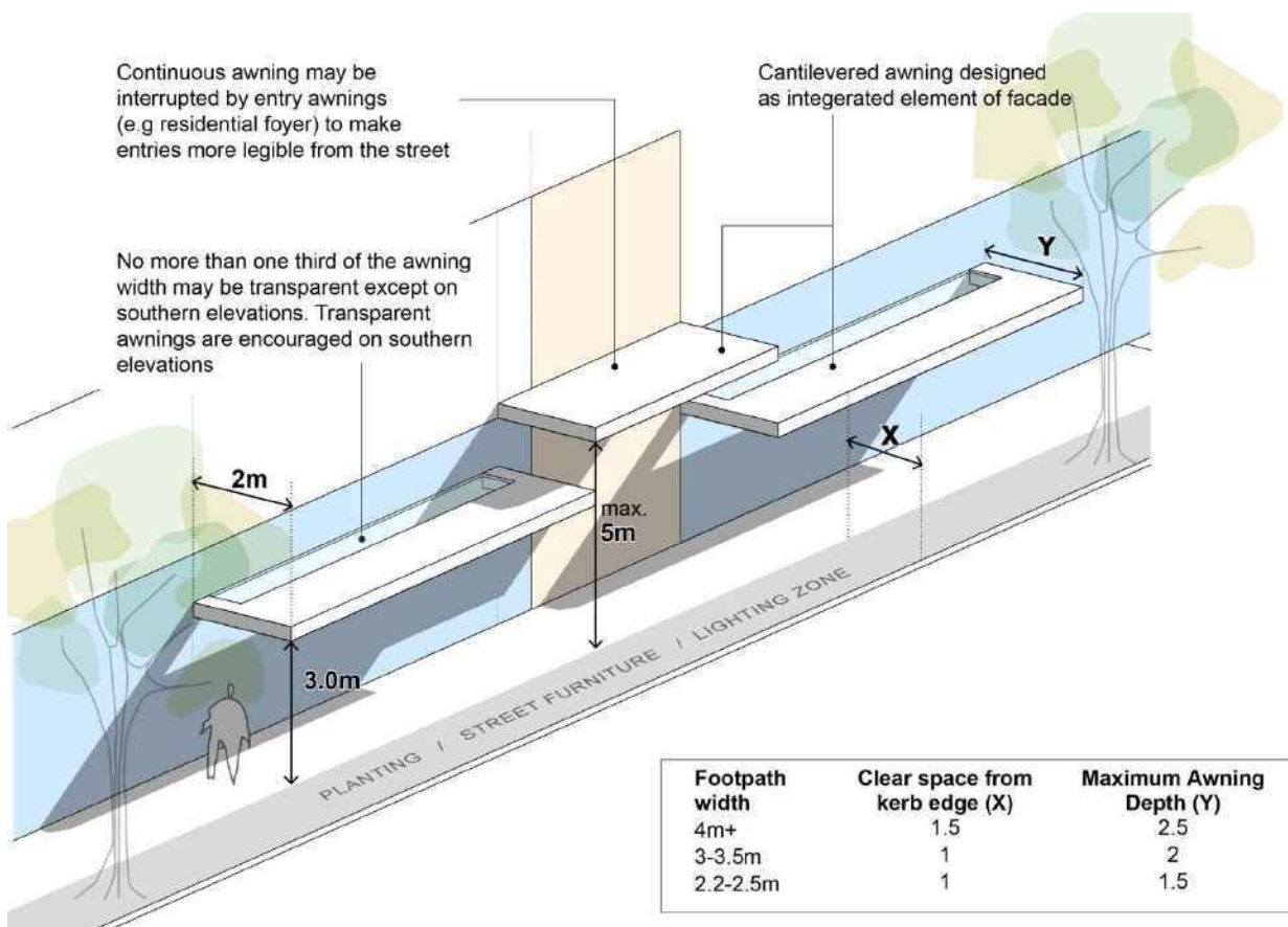
Figure E8.23: Awnings diagram
