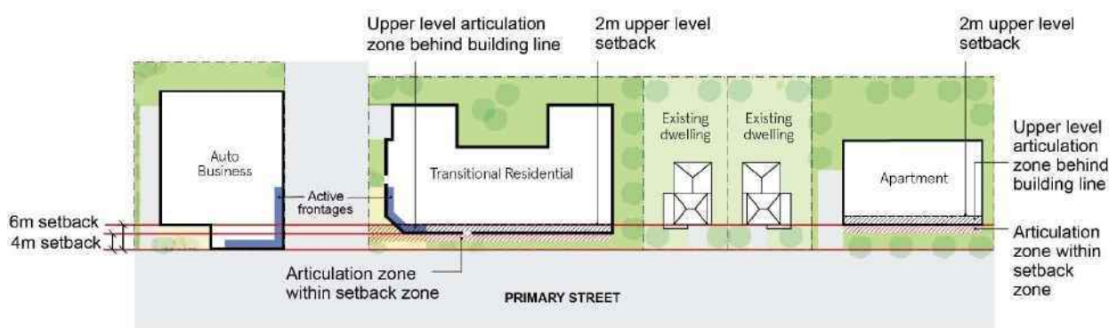
Figure F4E8.56: Front prevailing setback and articulation zone
