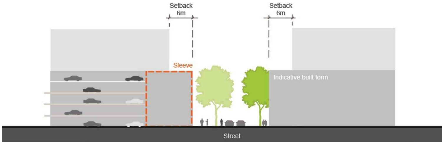
Figure F4E5.10: Sleeved car parking solution
