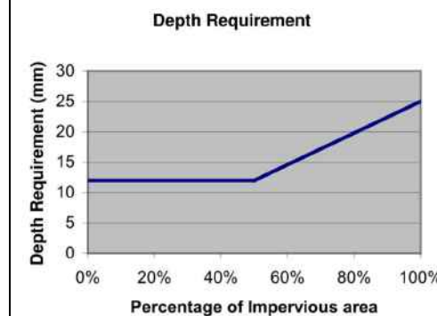
Figure C4.02: Impervious area to storage requirement relationship
