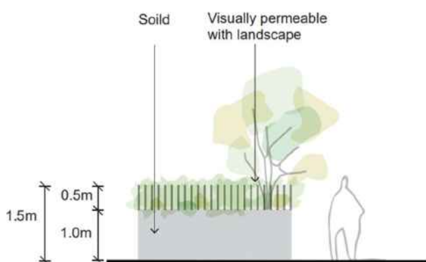
Figure F4E8.48: Active-residential fencing controls
