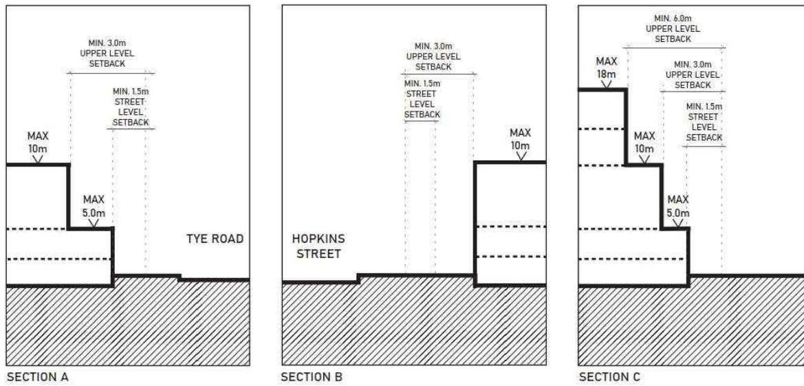
Figure F8E12.01: Cross sections A – C
