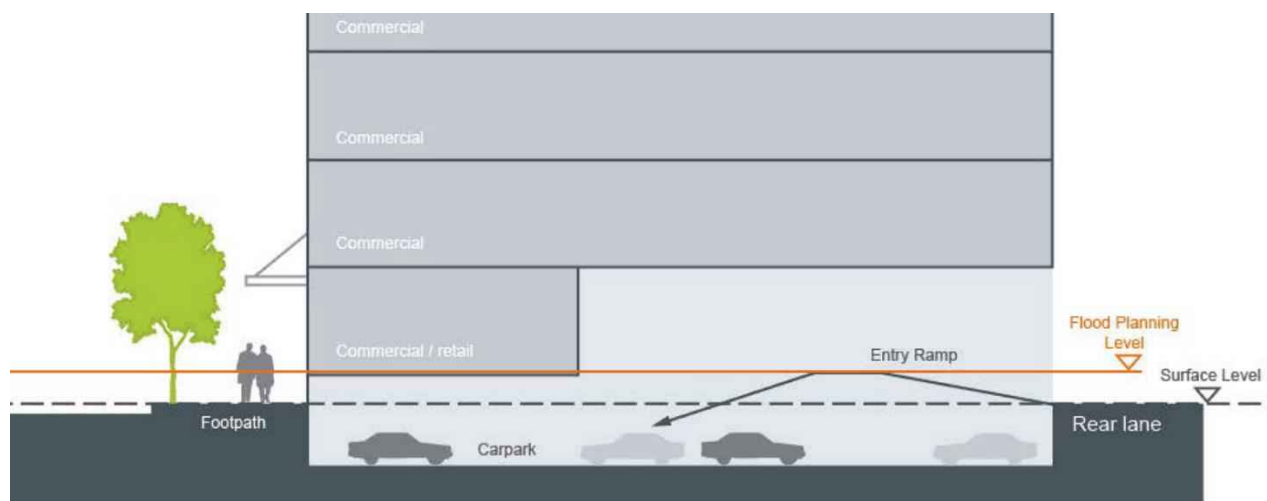
Figure F4E5.09: Basement ramp design to minimise flood inundation
