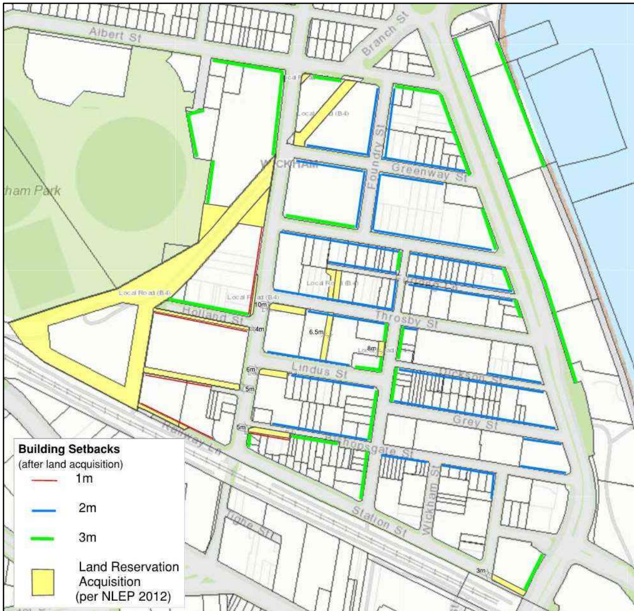
Figure F3E7.04: Ground level building setbacks to street boundaries
