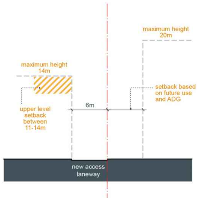
Figure E5.35: Section through Hunter Street live work units
