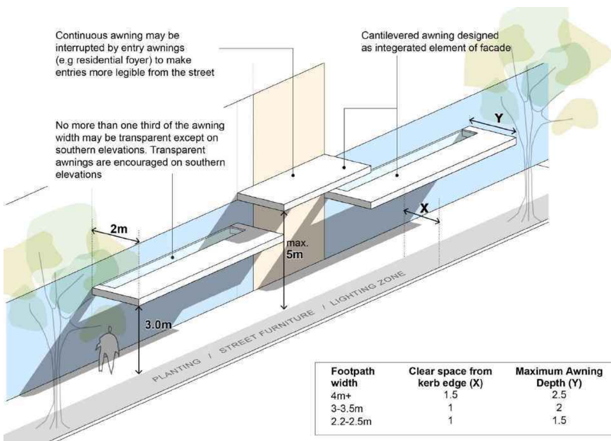
Figure F4E8.17: Awnings diagram
