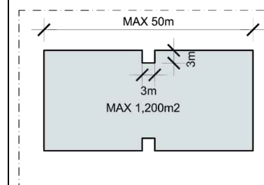
NON-RESIDENTIAL FLOORPLATE
