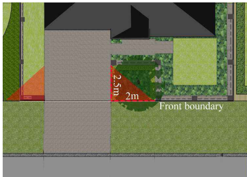
Figure D2.11: A 2m x 2.5m splay at the driveway and property boundary to avoid obstructions to visibility
