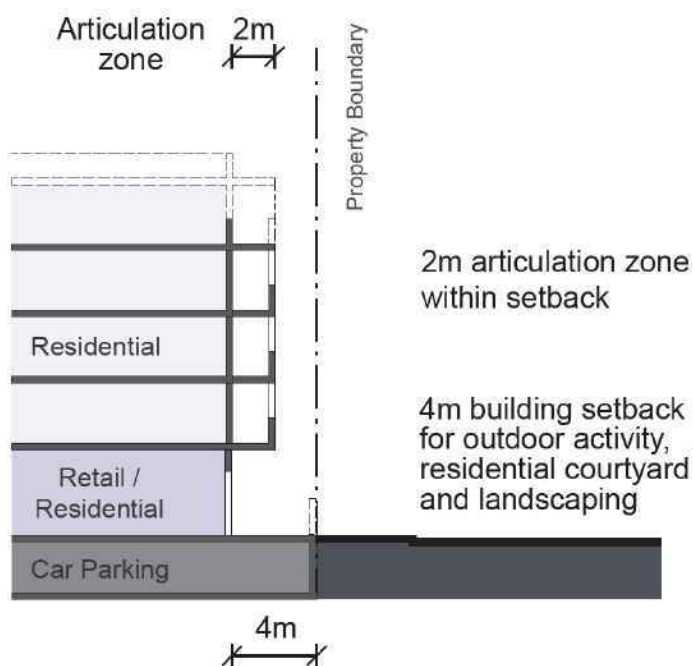
Figure F4E8.60: Setback transition - residential
