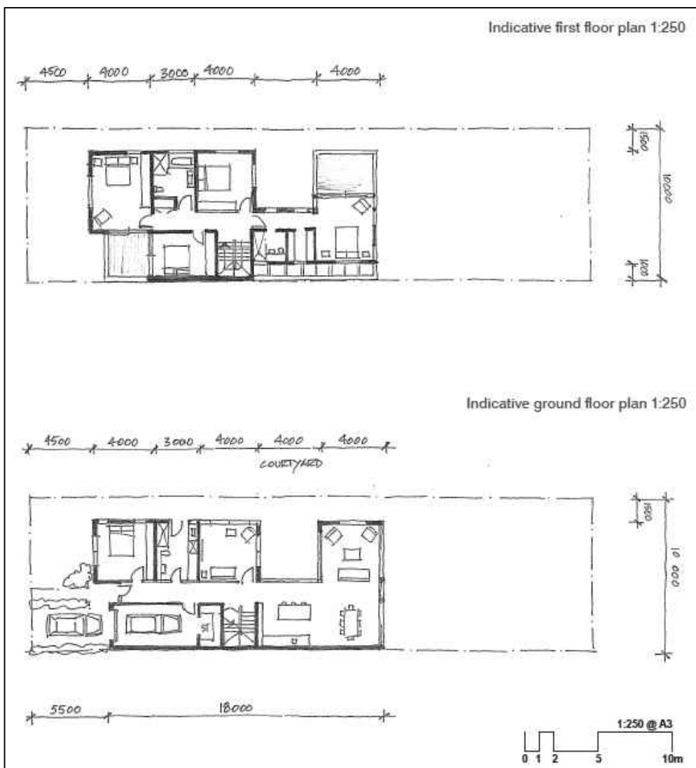
Figure F2E6.14: Courtyard housing typology
