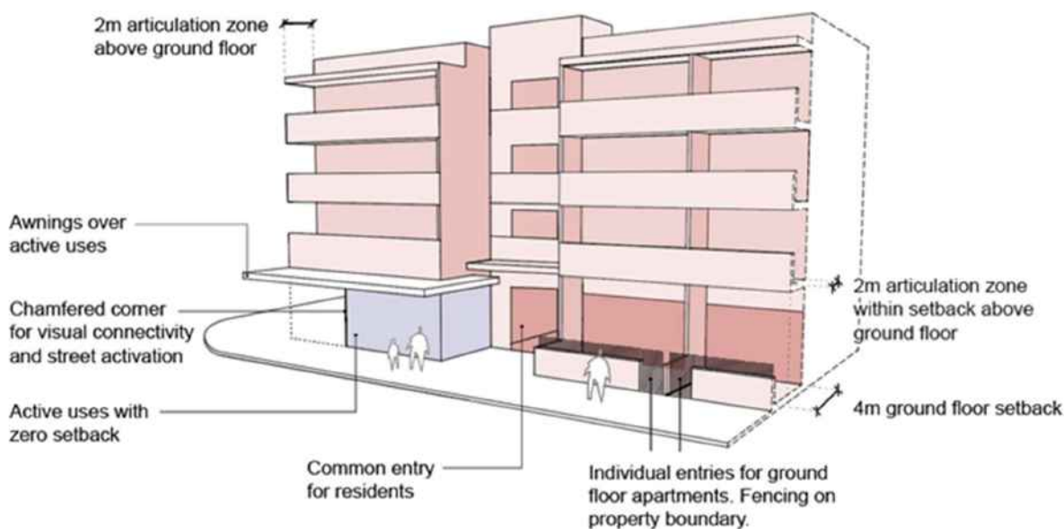
Figure F4E8.64: Non-residential and residential uses at ground level
