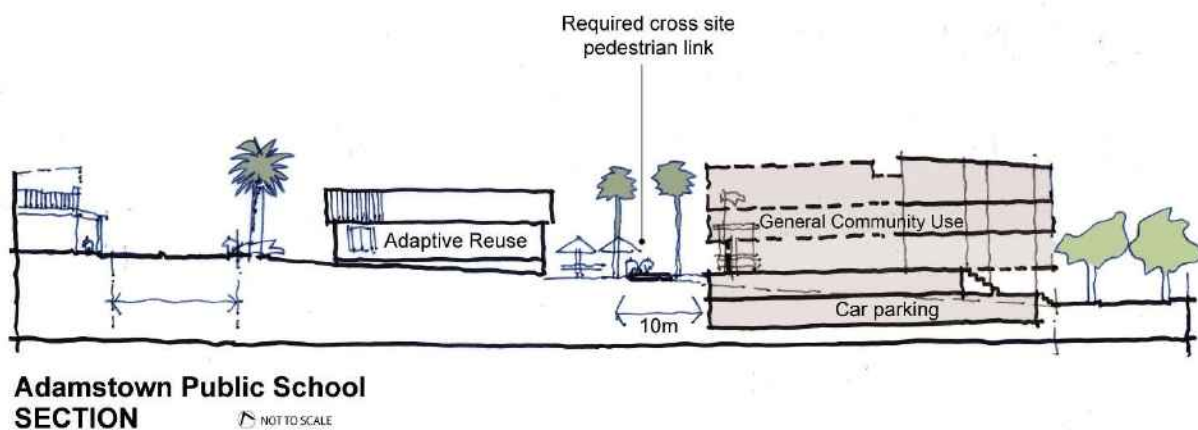
Figure F4E8.07: Adamstown public school section
