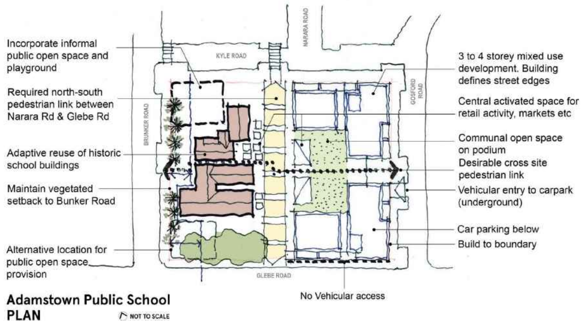
Figure F4E8.06: Adamstown public school plan
