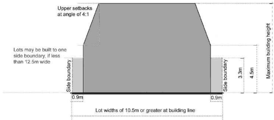
Figure D2.07: The following building envelope applies to lots with a width measured at the building line of 10.5m or greater
