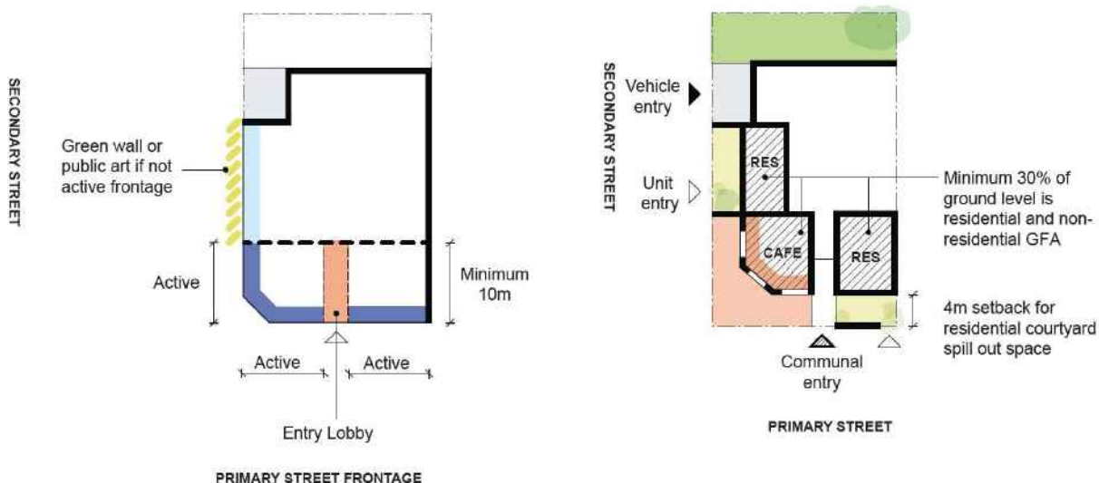
Figure F4E8.46: Ground level floor space and active frontages – Active-residential
