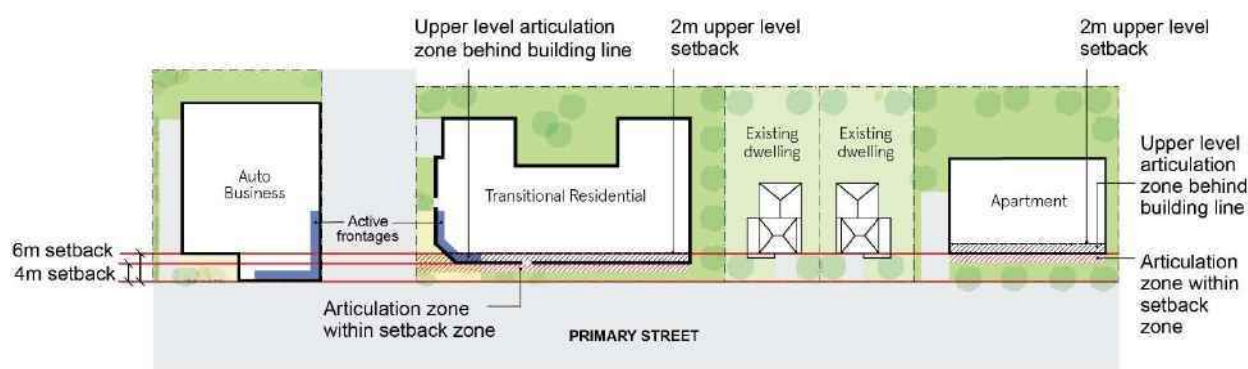
Figure F4E8.51: Front prevailing setback and articulation zone
