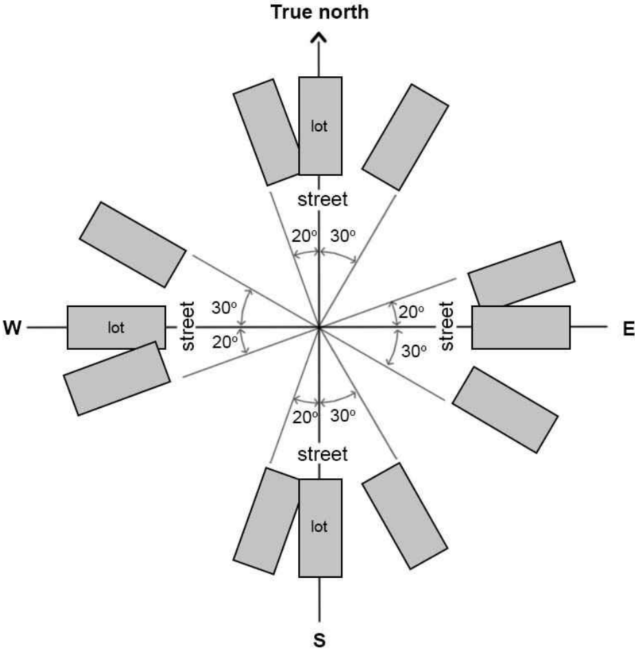
Figure D1.02: Preferred lot arrangement
