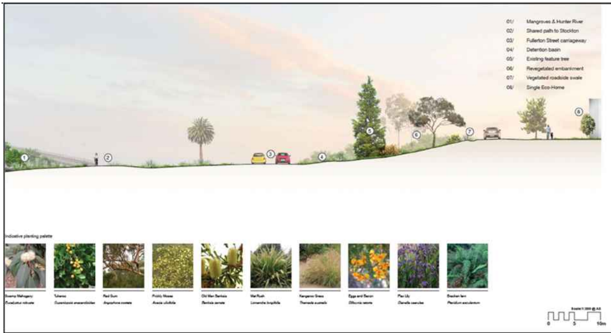
Figure F2E6.21: Frontage to Fullerton Street section
