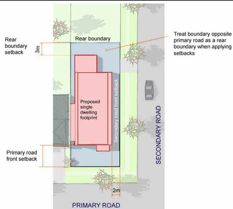
Figure D2.02: Setbacks from primary and secondary road
