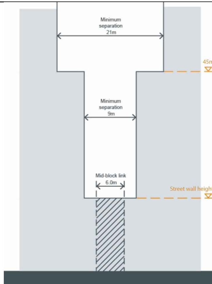
Figure F4E5.05 : Building separation for non-residential buildings within the same site
