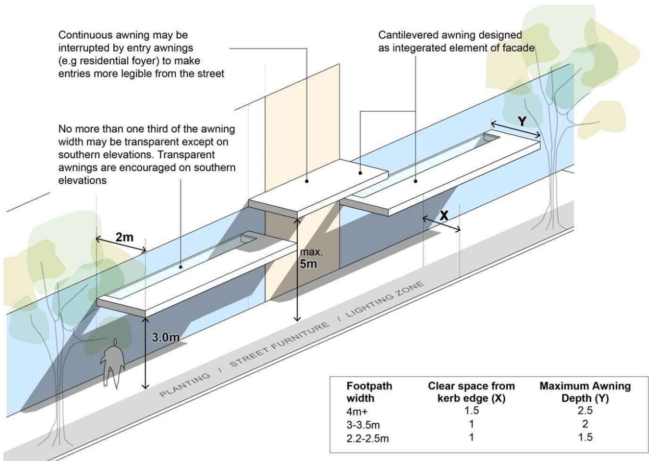
Figure E8.12: Awnings diagram
