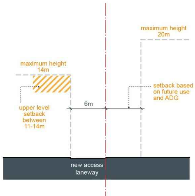
Figure F4E5.35: Section through Hunter Street live work units
