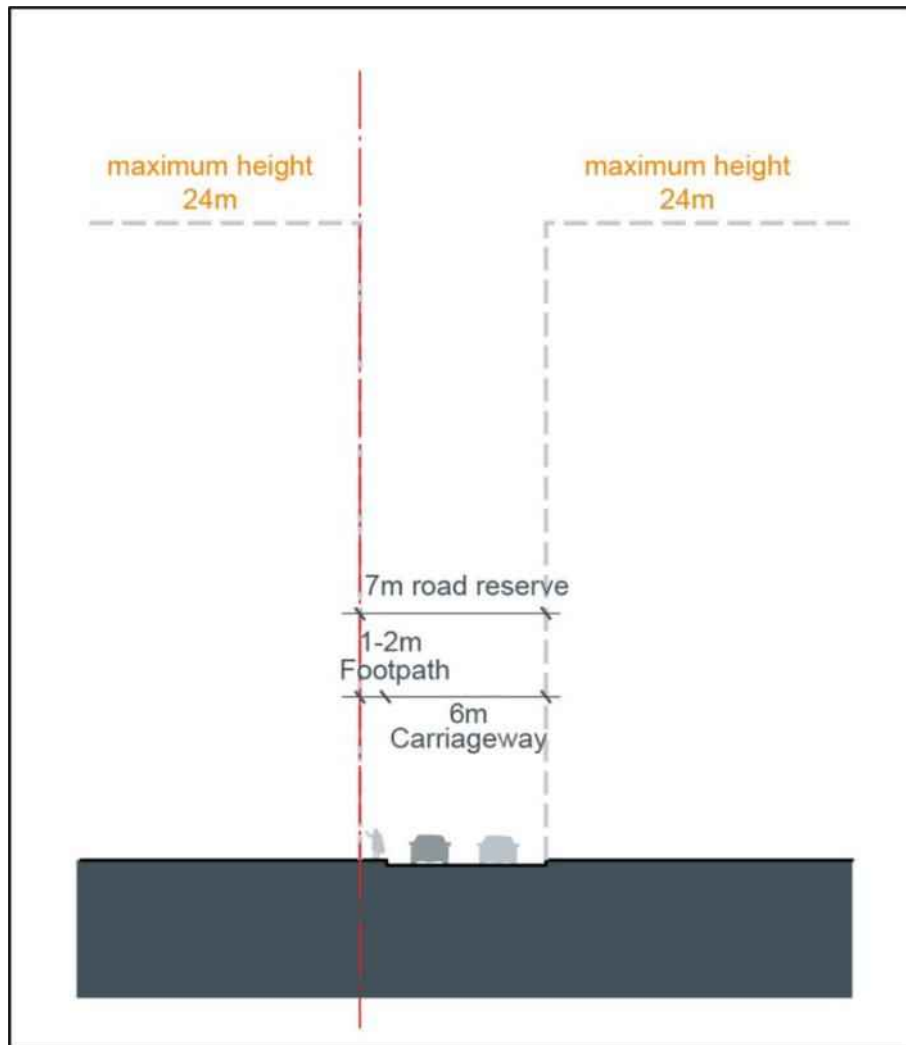
Figure F4E5.25: Civic lane section
