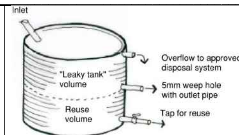
Figure C4.05 -- coastal: Coastal wetland rainwater tank configuration
