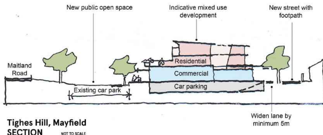
Figure F4E8.27: Section of landscape requirements for entry to corridor in Tighes Hill
