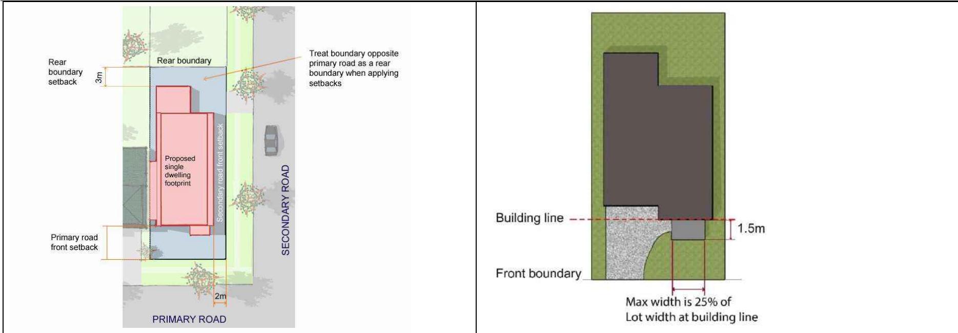
Figure D2.03: Aerial view of building articulation zone
