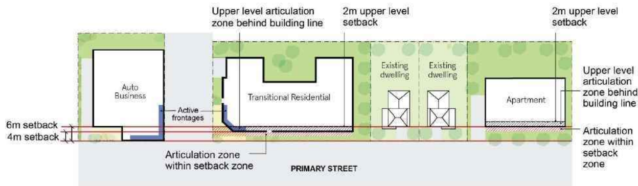
Figure F4E8.61: Front prevailing setback and articulation zone
