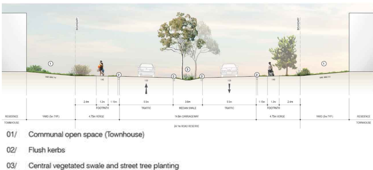
Figure E6.05: Road type 3 typical section
