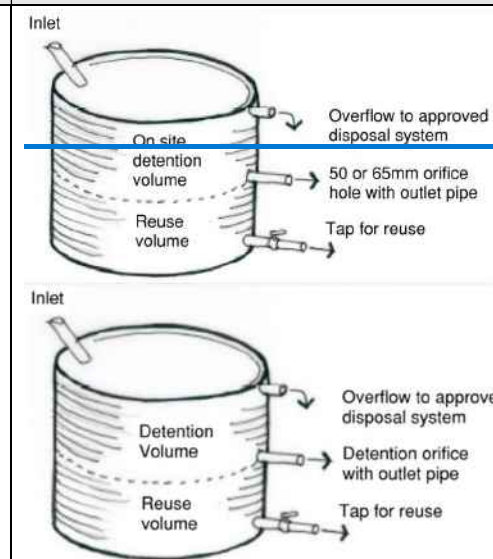
Figure C4.01: Example of above-ground tank with reuse and detention portions
