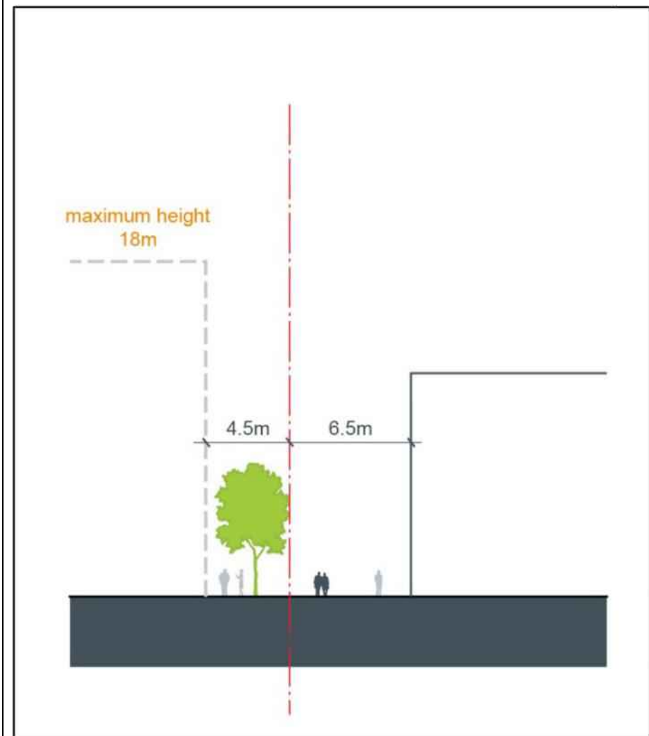
Figure F4E5.26: Section through new accessway way between Merewether Street and Civic Lane
