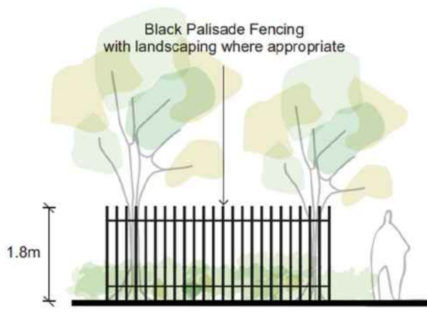
Figure F4E8.58: Non-residential fencing controls
