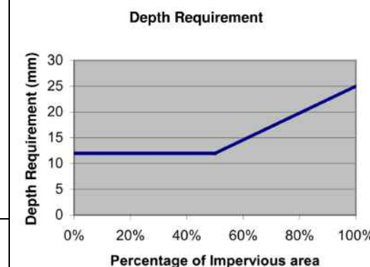
Figure C4.02: Impervious area to storage requirement relationship
