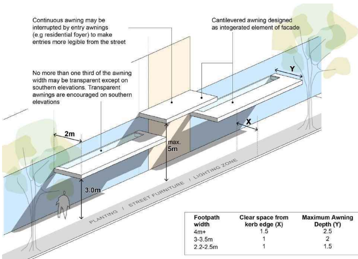
Figure F4E8.03: Awnings diagram
