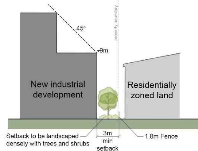
Figure D5.01: Setbacks to residential zoned land
