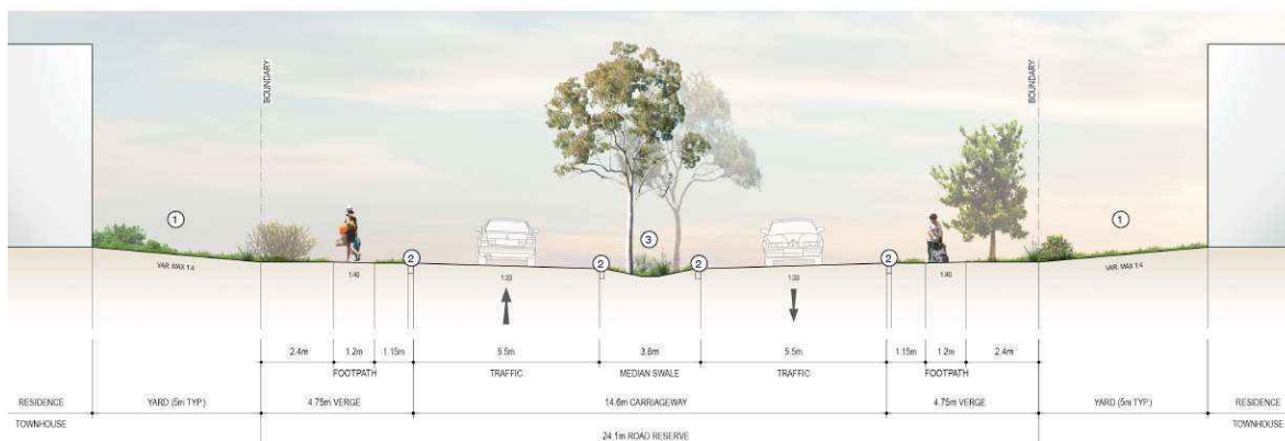
Figure F2E6.04: Road type 2 typical section
