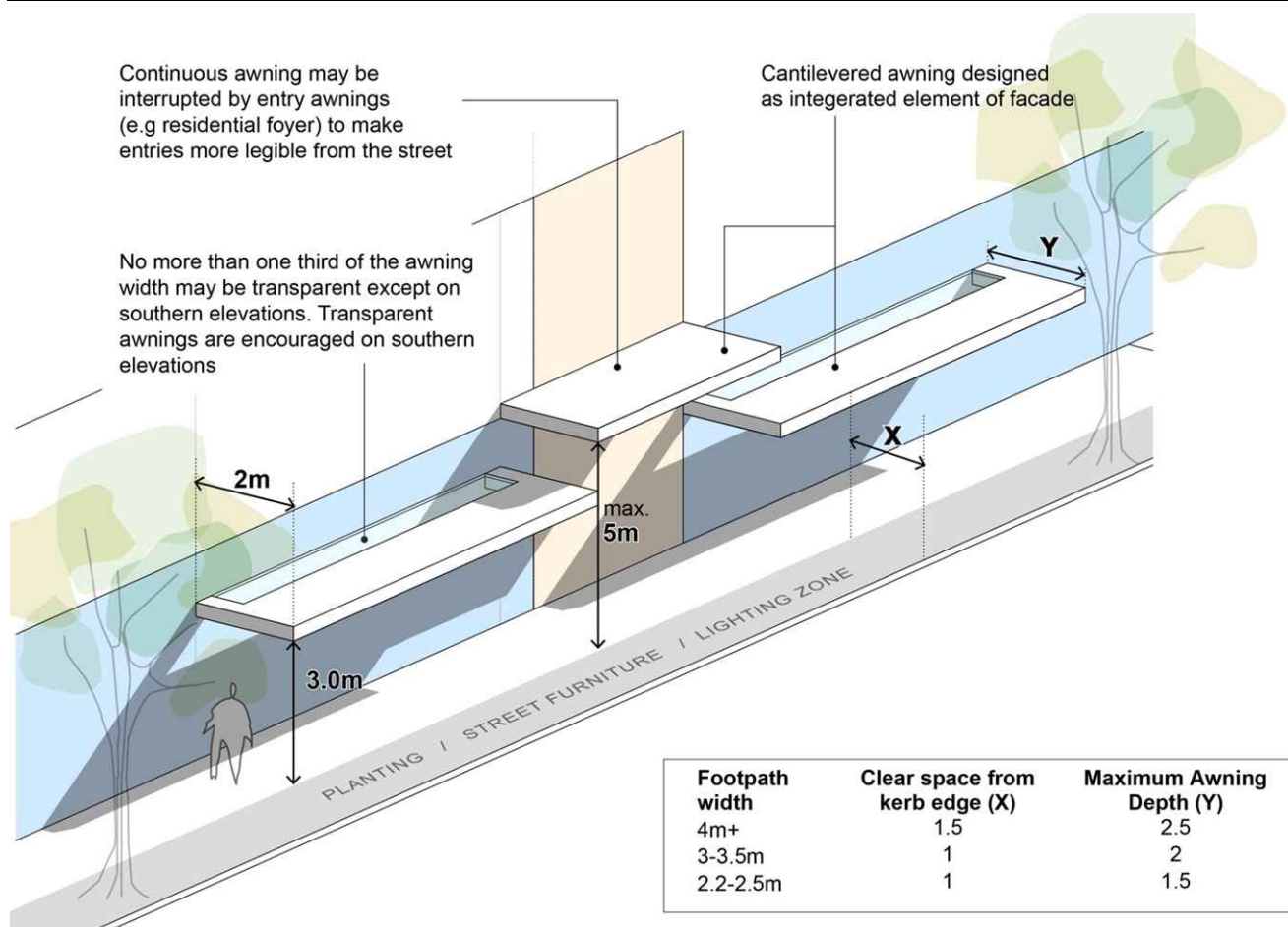
Figure C10.01: Awnings diagram
