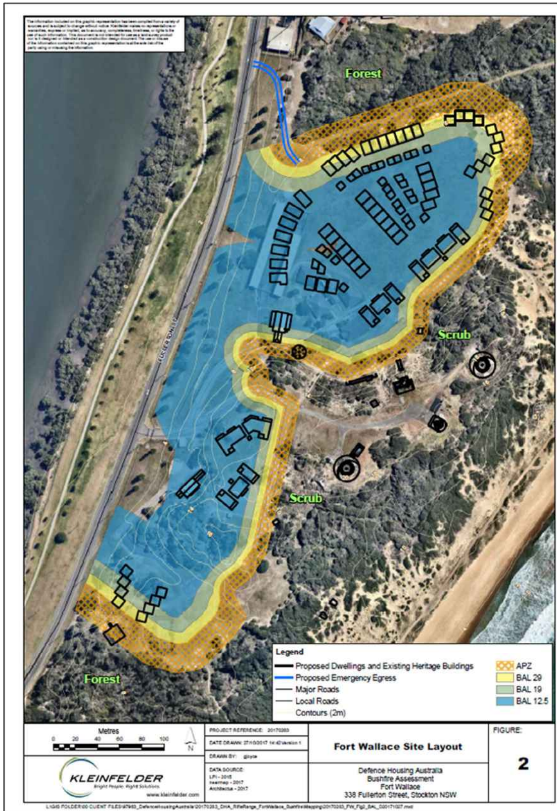
Figure F2E6.23: Asset protection zone
