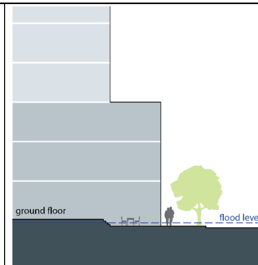
Figure F4E5.14: Floor level above flood level provided within building
