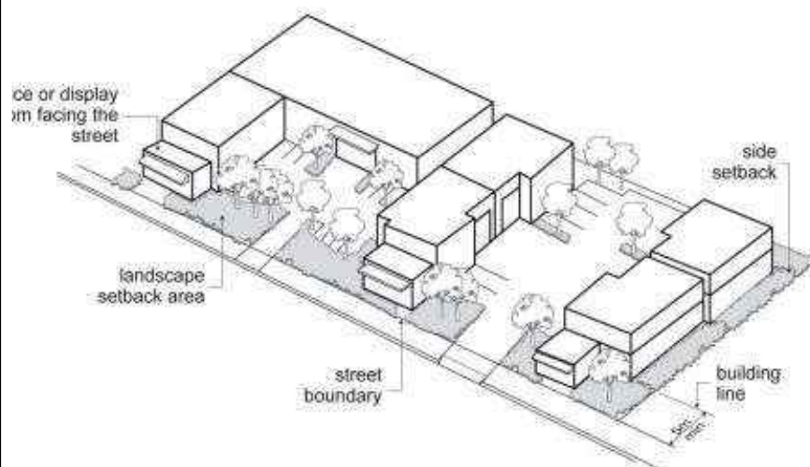
Figure D5.02: Street address and front setback
