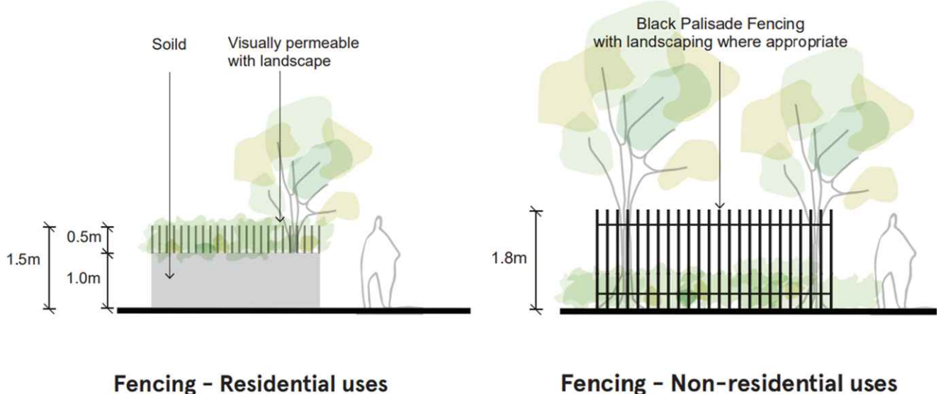
Figure E8.65: Fencing controls
