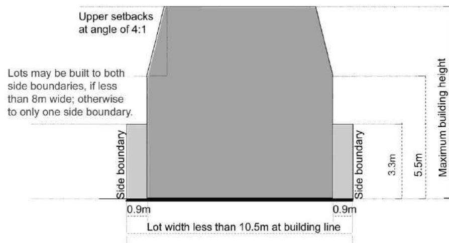
Figure D2.05: The following building envelope applies to lots with a width measured at the building line of less than 10.5m
