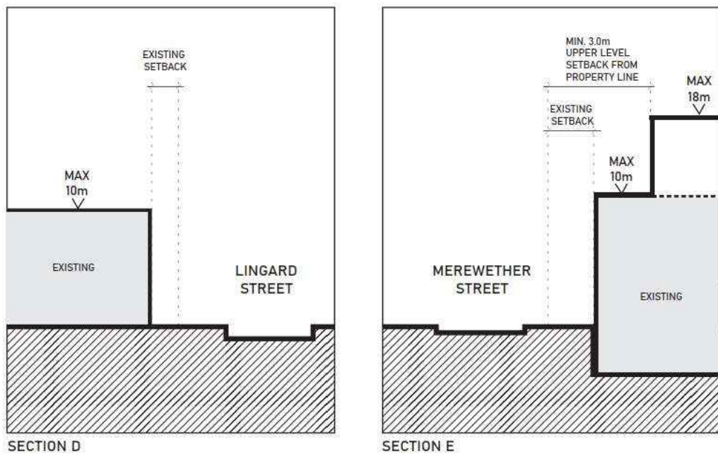
Figure F8E12.02: Cross sections D – E
