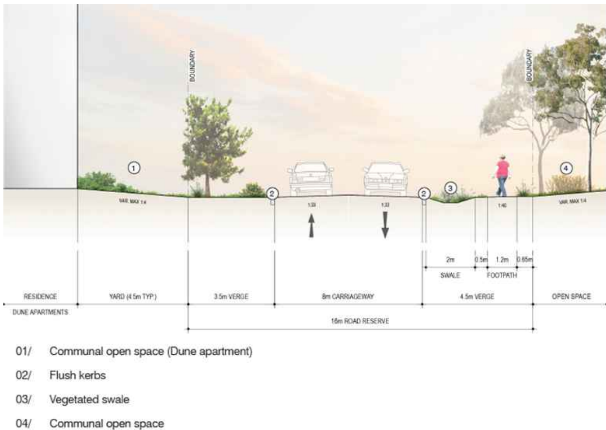
Figure E6.04: Road type 2 typical section
